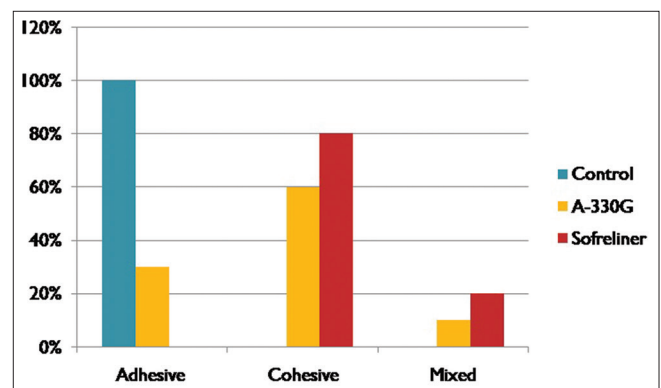
Figure 8: Mode of failures in the fiber-reinforced composite group
